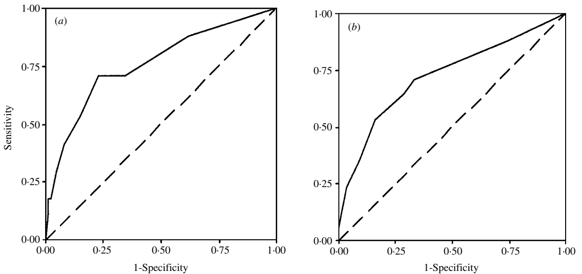
FIG. 2. ROC curves of (a) number of inattentive symptoms and (b) number of hyperactive-impulsive symptoms versus 95th percentile cutoff of impairment.
